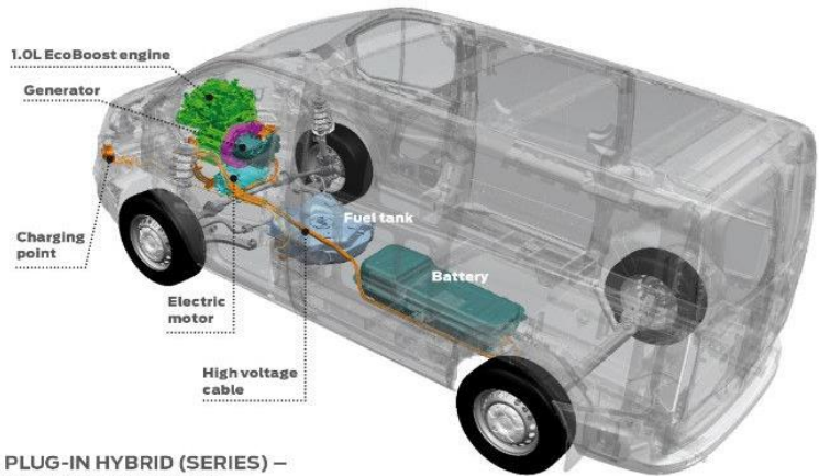
PLUG-IN HYBRID (SERIES) – Transit Custom PHEV
